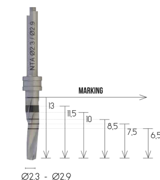
Tapered Drill
