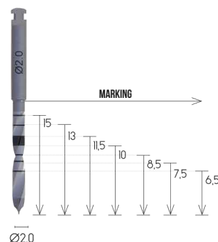
Guide Drill
